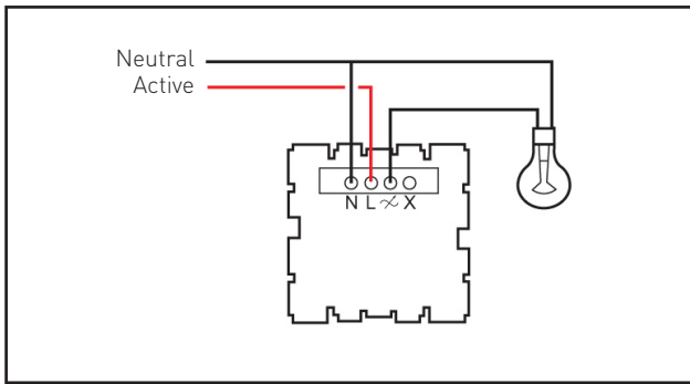
One-way wiring
