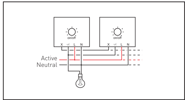
Multi-way wiring (maximum of 5 switches)
